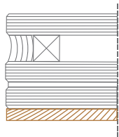
Isolant, marbre extérieur Insulated, marble outside
