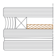
Isolierglas, marmor innen hohlraum Insulated, marble inside cavity
